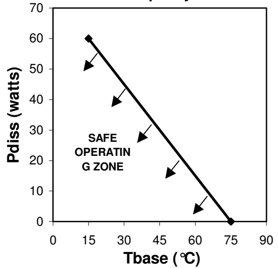
High power package dissipation capacity
