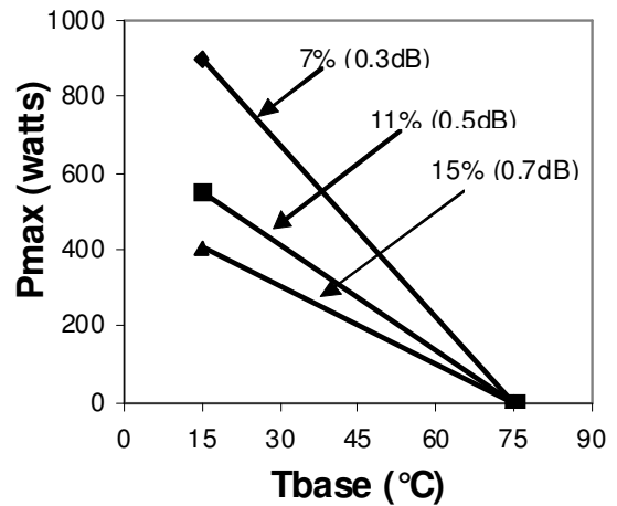
MAXIMUM ALLOWABLE INPUT POWER FOR ALL PORTS TOGETHER GIVEN DIFFERENT INSERTION LOSS
