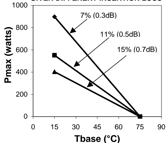
MAXIMUM ALLOWABLE INPUT POWER FOR ALL PORTS TOGETHER GIVEN DIFFERENT INSERTION LOSS
